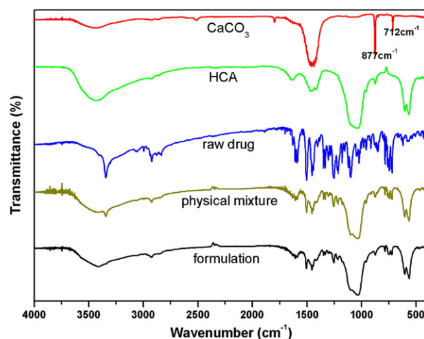
Fig. 7. The FTIR spectra of CAR, pure HA, physical mixture and HCA-3-1.
