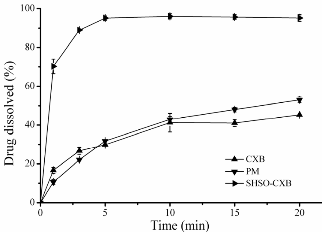
Figure 8. The dissolution profiles: raw CXB; PM; SHSO-CXB, n=3
