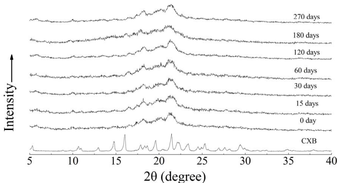
Figure 7. XRPD patterns of SHSO-CXB on different days under storage at room temperature
