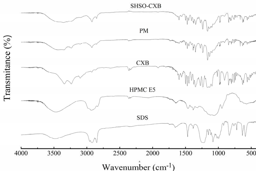
Figure 6. FT-IR spectra: raw CXB; PM; SHSO-CXB and stabilizers (HPMC E5 and SDS)
