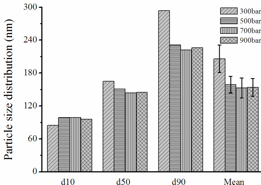
Figure 2. Volume-weighted PSD of CXB nanoparticles prepared under different homogenization pressures (CXB concentration: 60 mg/ml; stabilizer concentration: 0.15%, w/v; acetone/water volume ratio: 1/20; 15 cycles), n=3
