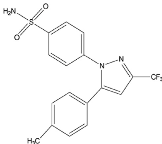
Figure 1. Chemical structure of CXB
