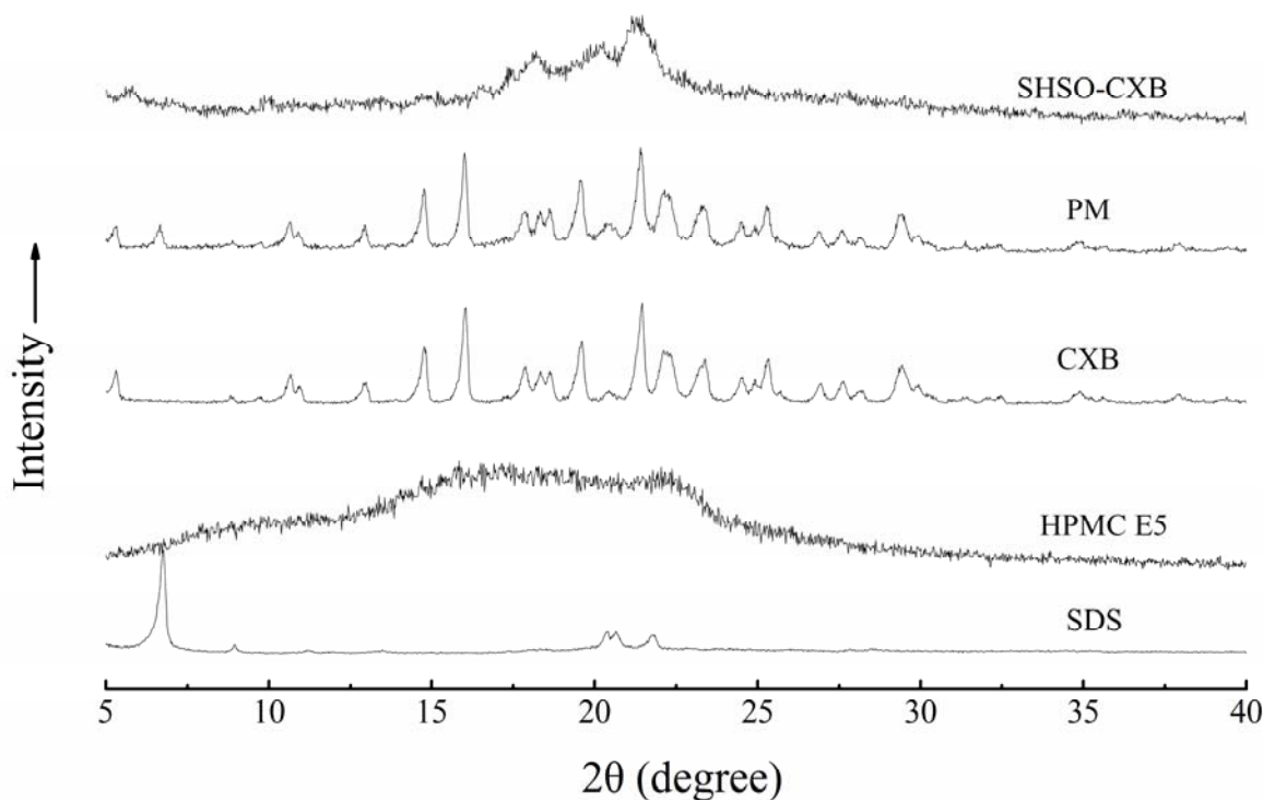
Figure 5. XRPD patterns: raw CXB; PM; SHSO-CXB and stabilizers (HPMC E5 and SDS)
