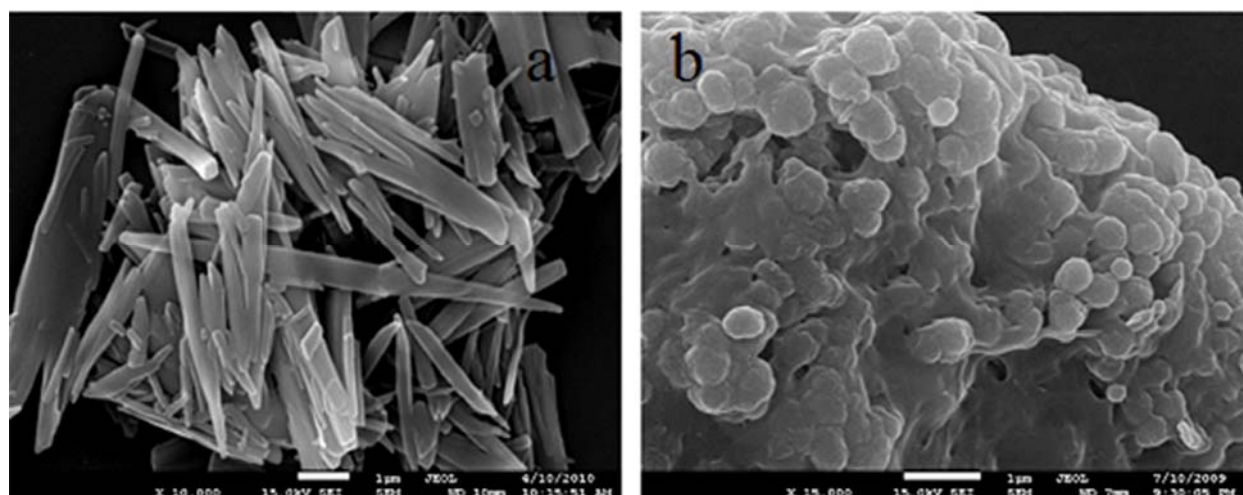
Figure 3. SEM images of raw CXB (a) and CXB nanoparticles (b)
