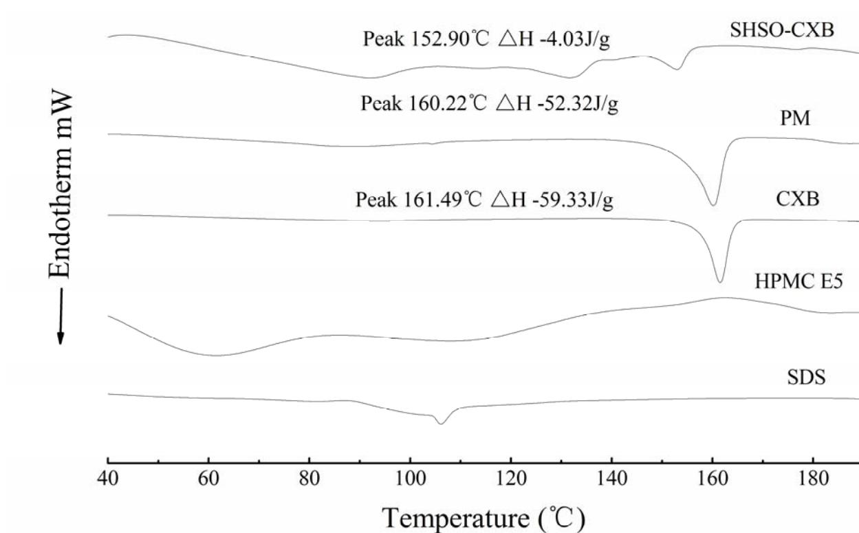
Figure 4. DSC curves: raw CXB; PM; SHSO-CXB and stabilizers (HPMC E5 and SDS)
